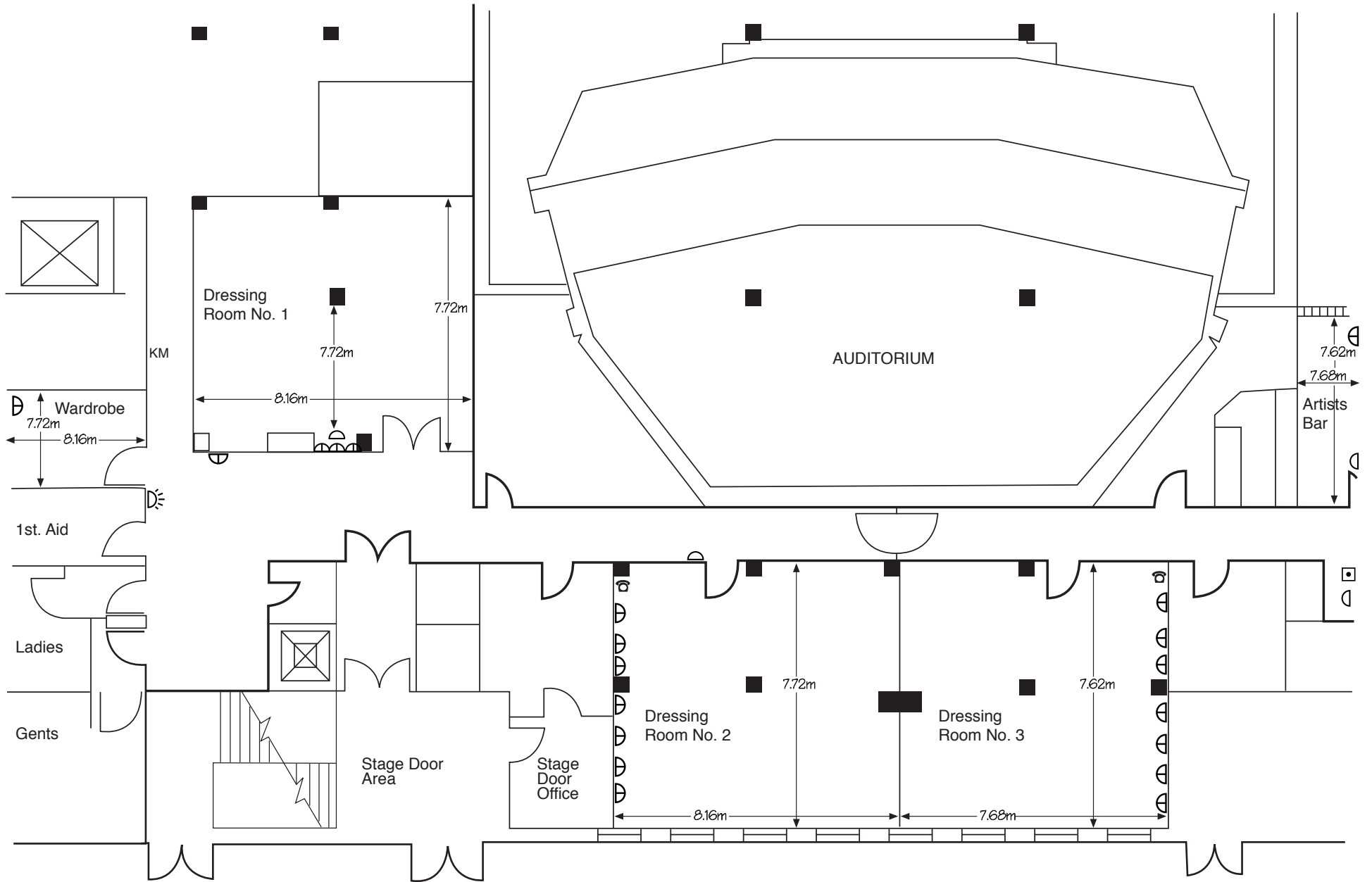
Dressing Rooms No. 1, 2 & 3 on Level 0.
